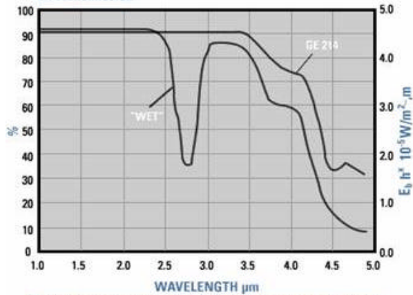
IR Transmission
