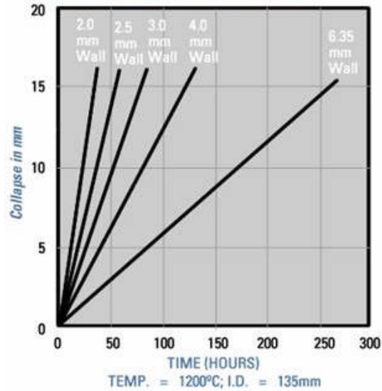
Diffusion Tubing, Collapse vs. Time for Wall Thickness
