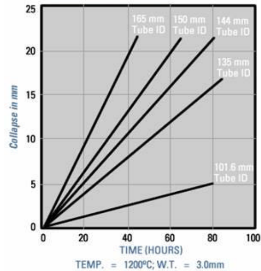
Diffusion Tubing, Collapse vs. Time for Tube ID
